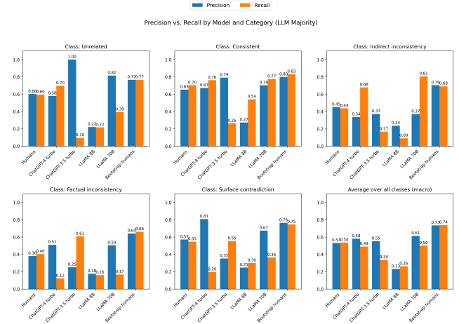
Figure 6: Precision and Recall distribution for 5 classes.
