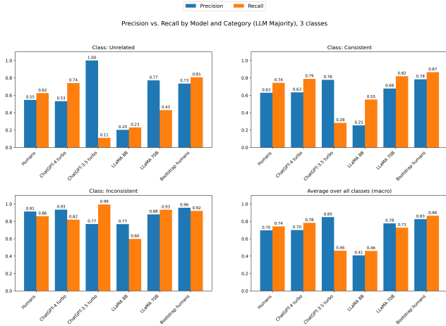
Figure 5: Precision and Recall distribution for 3 classes.
