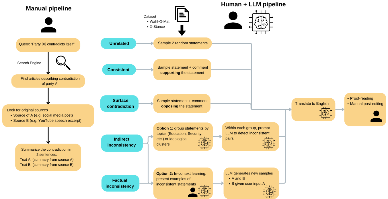
Figure 2: Schematic description of the data annotation pipelines.
