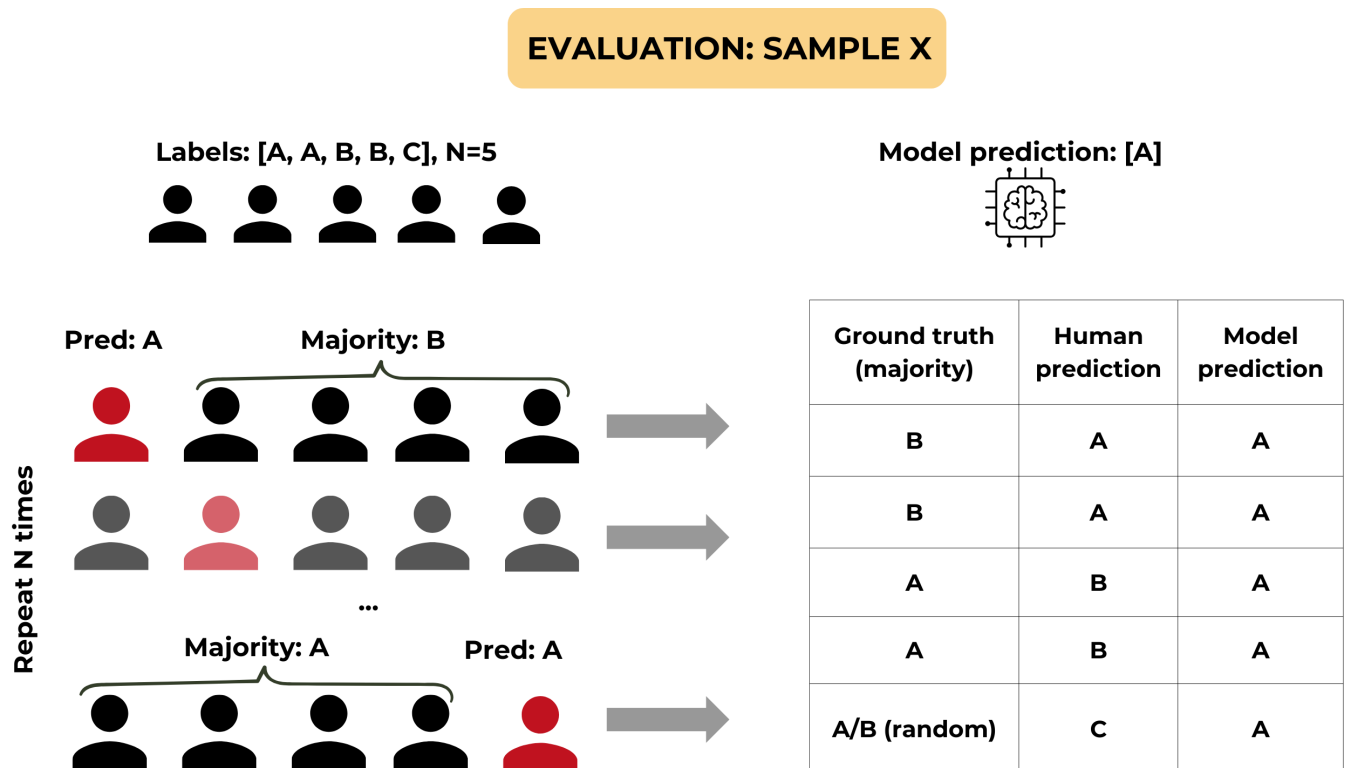
Figure 16: A scheme for evaluating individual humans and models' prediction of the majority label.
